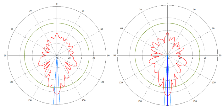
Horizontal polarization
