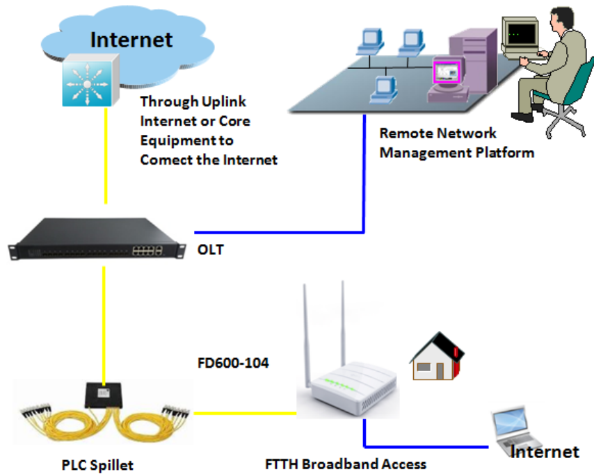
Figure: FD600-104 Application Diagram
