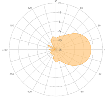
N5-X12 (12 dBi)
